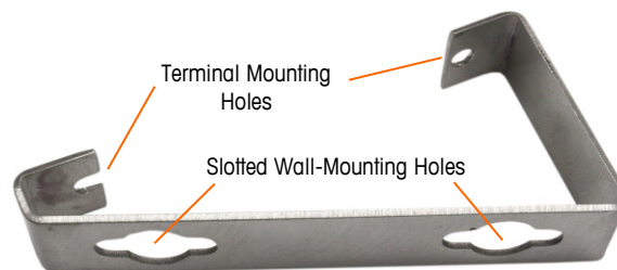
Figure 2-10: Wall-Mounting Bracket
